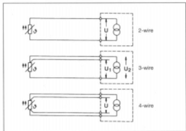
Fig. 21: Connection of resistance thermometers
