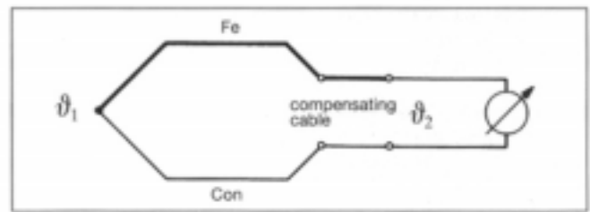
Fig.4: Thermocouple with compensating cable
